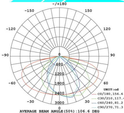
Photometric data
