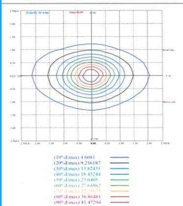
ISO illuminance diagram [Unit:lx]
